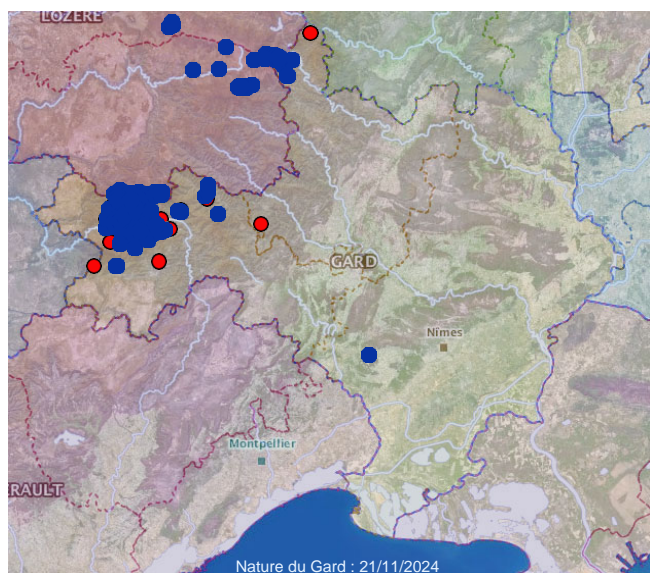
1 - Lycaena virgaureae (Linnaeus, 1758)
