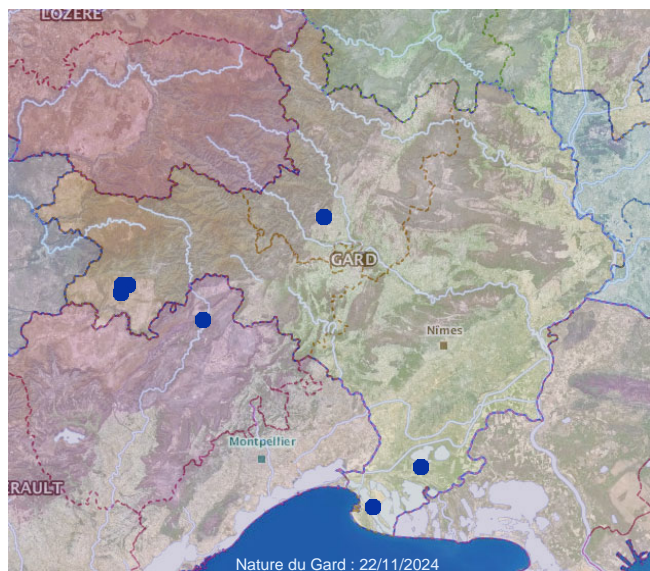
1 - Procrinae Boisduval, 1828
