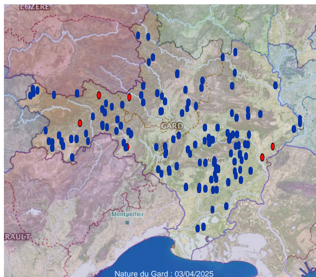
1 - Polyommatus Latreille, 1804
